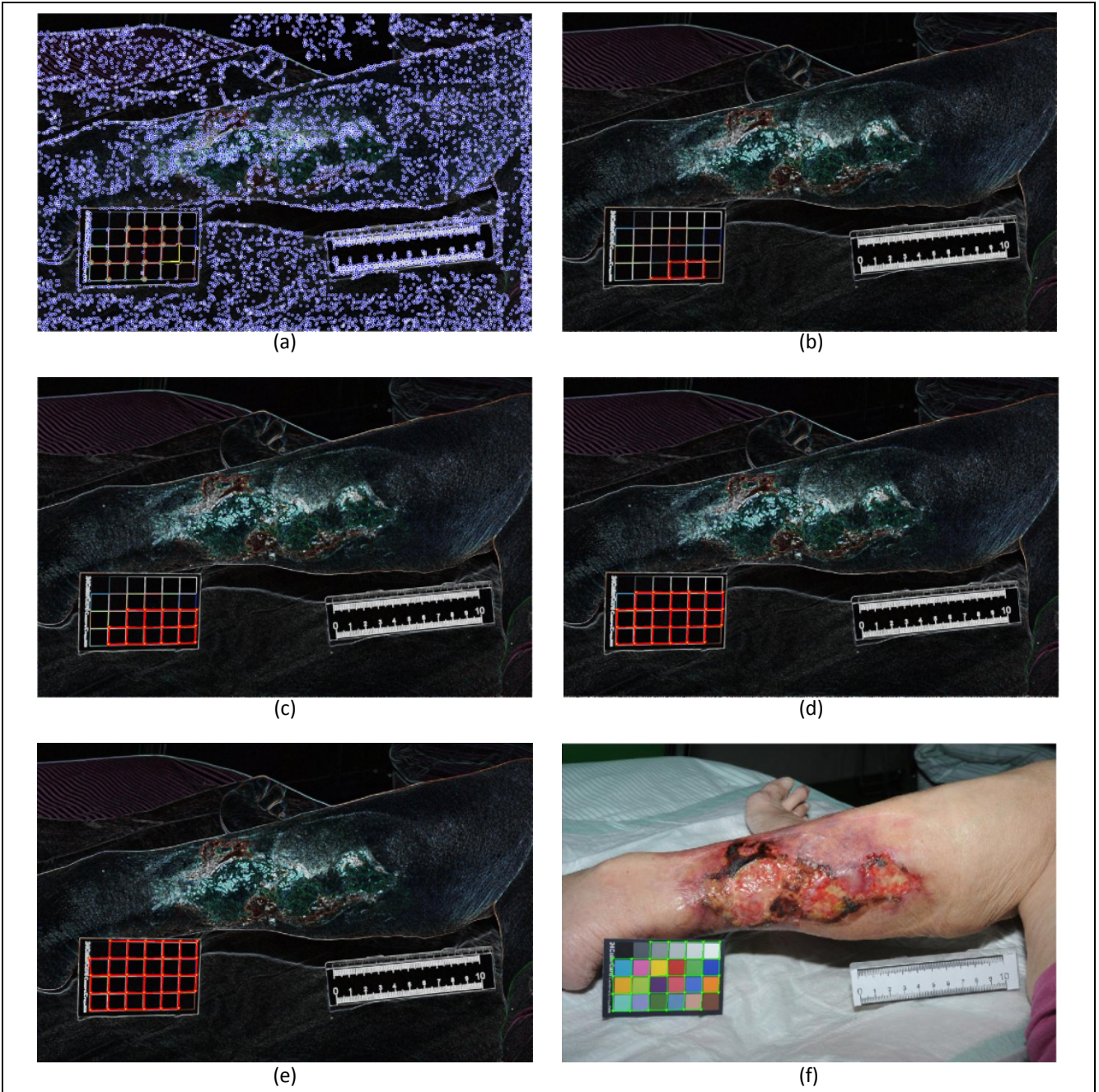
Figure 1: Stages of the lattice detection process. Edge map with feature points and selected candidate points of lattice (a); iterative process of lattice detection (b) – (e); and final lattice grid superimposed on the original photograph (f).
